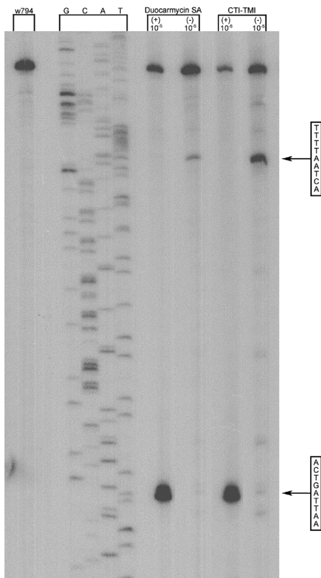
Figure 3. Thermally-induced strand cleavage of w794 DNA (144 bp, nucleotide no. 5238–138) after DNA-agent incubation with duocarmycin SA and CTI-TMI (24 h, 23 °C), removal of unbound agent by EtOH precipitation and 30 min thermolysis (100 °C), followed by denaturing 8% PAGE and autoradiography. Lane 1, control DNA; lanes 2–5, Sanger G, C, A, and T sequencing standards; lane 6, (+)-duocarmycin SA ( 1 \times 10^{-5} M); lane 7, (-)-duocarmycin SA ( 1 \times 10^{-5} M); lanes 8 and 9, (+)-CTI-TMI and ent -(-)-CTI-TMI ( 7 , 1 \times 10^{-5} M).
